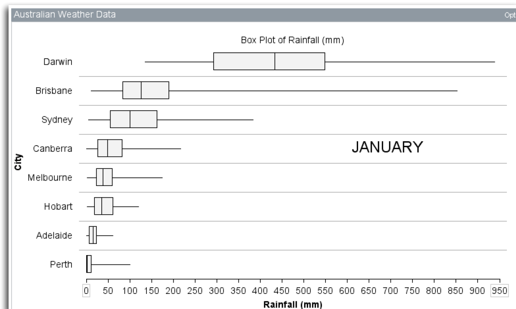
January Rainfall for 56 Years
