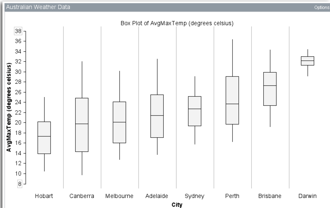
Average monthly maximum temperature for 56 years
