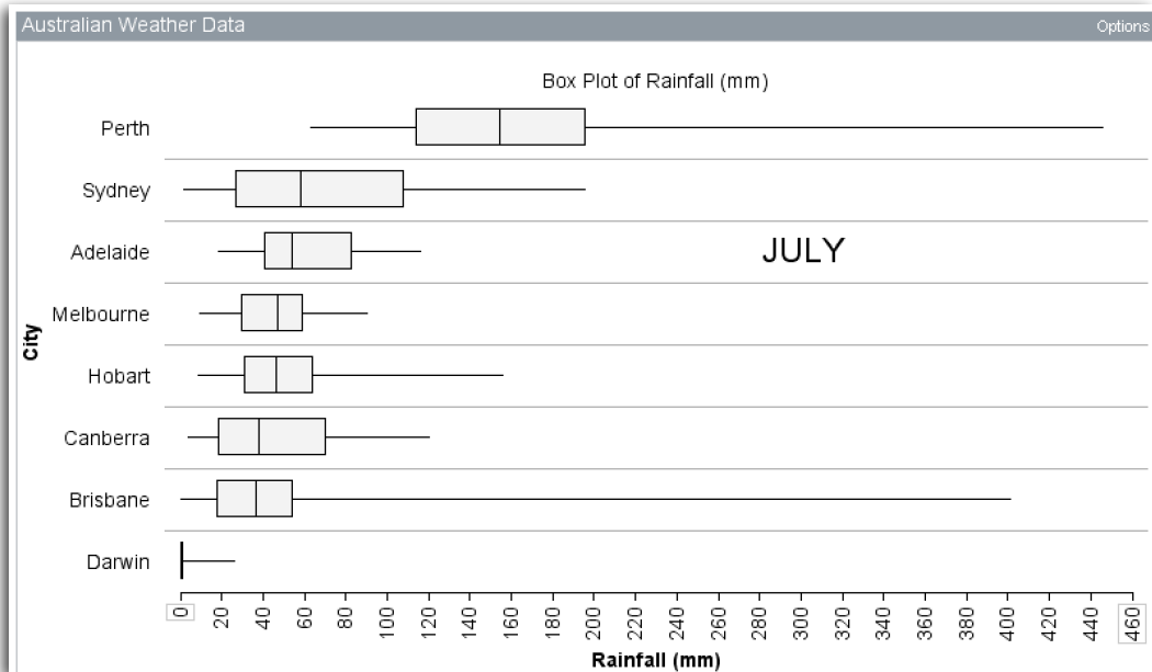
July Rainfall for 56 Years
